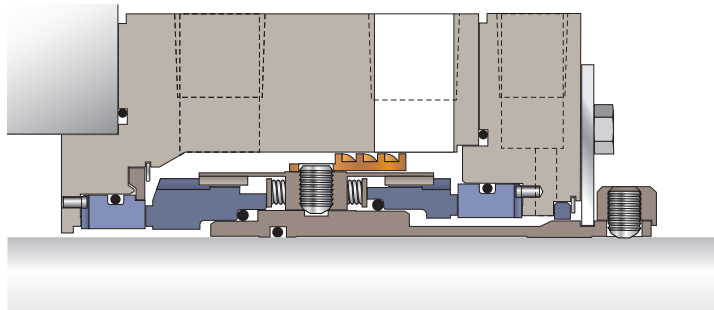
Arrangement 3 QB2B/QB back-to-back pressurized dual seal with barrier fluid provides zero emissions sealing
