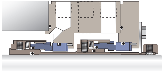
Arrangement 2 QBQ/QBQ unpressurized dual seal with liquid buffer fluid provides near-zero emissions sealing
